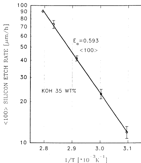
Fig. 4: Temperature dependence of [100] oriented etch rate for 35wt% KOH solution
