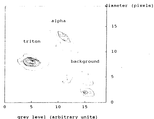
Fig. 5: Bright areas on the diagram correspond to large number of tracks with given size (y coordinate) and average grey level (x coordinate).
