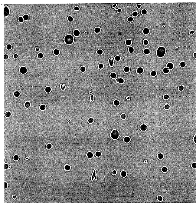
Fig. 3: Ellipse fitting to the tracks. Program is capable to fit correctly even the overlapping tracks.
