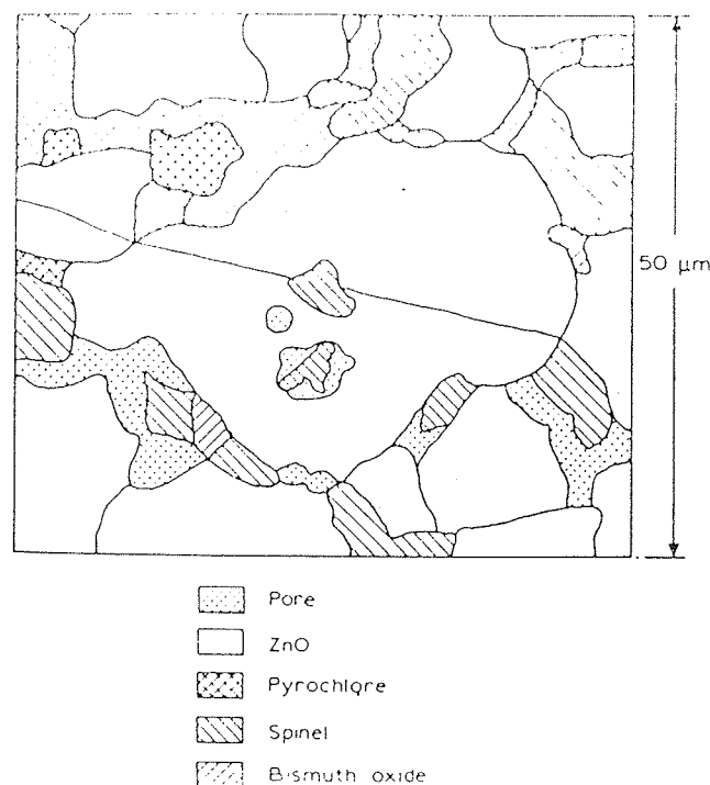
Figure 2: Actual structure of ZnO varistor 7
