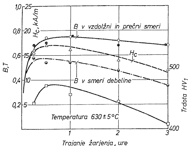
Fig. 5: Fe_{30}Cr_{10}Co alloy. Effect of annealing for spinodal decomposition at 630^{\circ}C on coercivity, remanence and hardness. The alloy was homogenised at 1200^{\circ}C and quenched.
