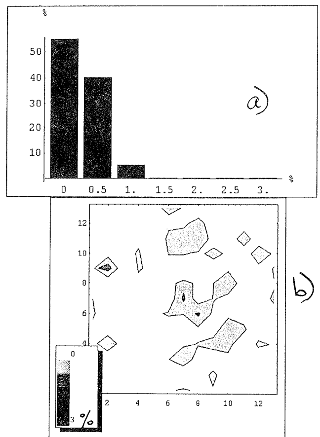
Fig. 23: Polysilicon sheet resistivity matching a) histogram and b) on wafer uniformity in %. Two neighbouring polysilicon resistors with same dimensions, L = 200 \mu\text{m} , W = 20 \mu\text{m} .
