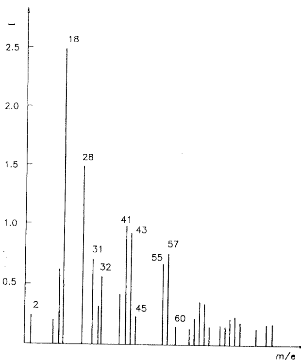
Fig. 4: Mass spectrum of the outgassing products from the electrochemically gold plated (citrate and phosphate electrolyte) contact alloy Argelec 181 ( 135^\circ\text{C} , 1 \times 10^{-6} mbar) after 30 minutes of outgassing.
