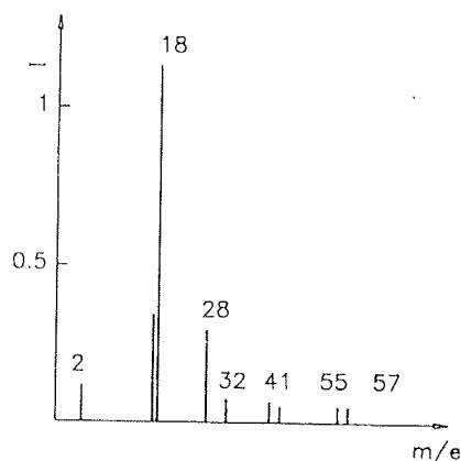
Fig. 3: Mass spectrum of the outgassed empty chamber ( 150^\circ\text{C} , 24 hours of outgassing).
