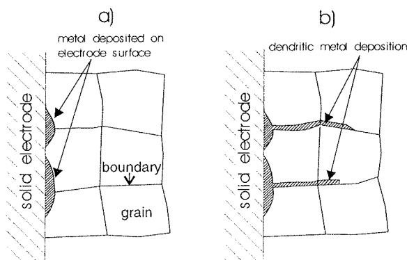
Fig. 6: a) deposition of metallic lithium in the first stage of dc voltage application, b) deposition of Li at after prolonged application of dc voltage.
