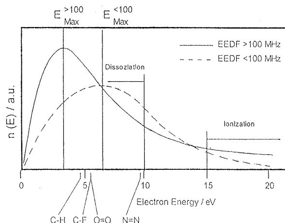
Figure 10: EEDF as a function of plasma excitation frequency
