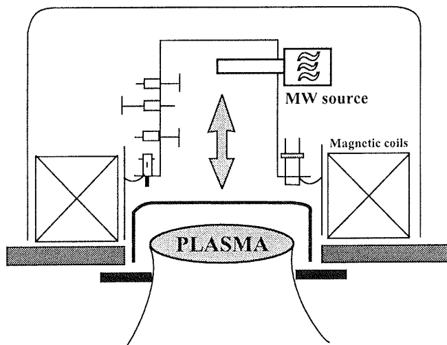
Figure 15: ECR plasma stream source
