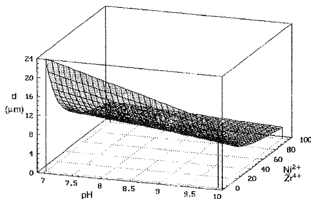
Fig. 3: Average particle size profile of precipitated composites as a function of final pH in the reaction mixture and initial molar ratio \text{Ni}^{2+}/\text{Zr}^{4+}
