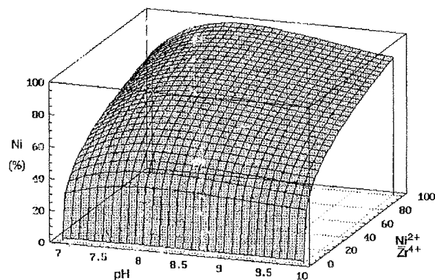
Fig. 4: Chemical composition of finally prepared composites as a function of final pH in the reaction mixture and initial molar ratio \text{Ni}^{2+}/\text{Zr}^{4+}
