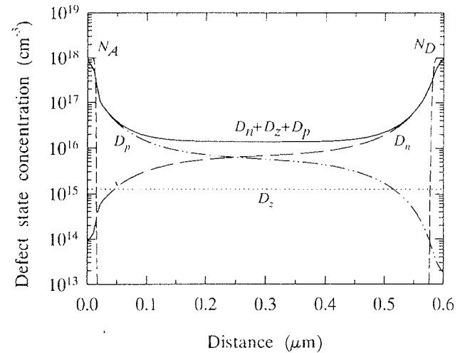
Fig. 4: Defect pool in the p-i-n structure: calculated distribution of defects D_n , D_i , D_p and the doping profile.
