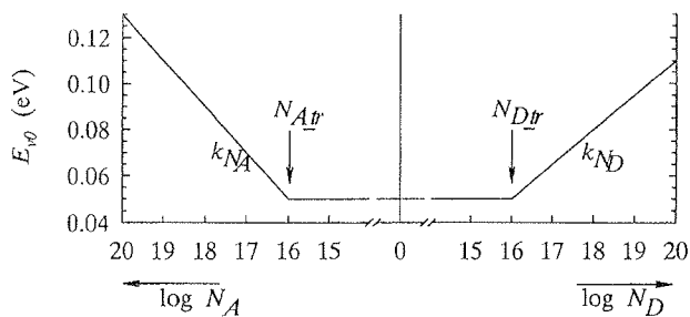
Fig. 6: A model of E_{v0} dependency on doping concentration. Similar dependency holds also for E_{c0} - only initial value E_{c00} is smaller (25 meV).
