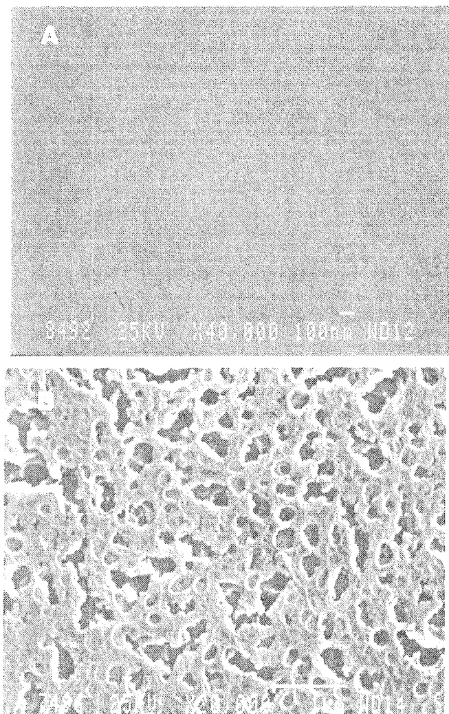
Fig. 1: Morphology of undoped \text{TiO}_2 thin films fired at 650^\circ\text{C} for 1 h. A: NK/P0.0, B: NK/P2.4
