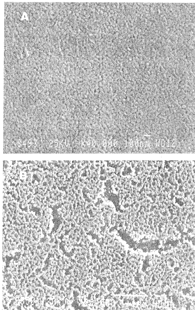
Fig. 2: Morphology of potassium doped \text{TiO}_2 thin films fired at 650^\circ\text{C} for 1 h. Samples were prepared from \text{KOOCCCH}_3 and \text{KNO}_3 doped sols. A: KA/P2.4, B: KN/P2.4
