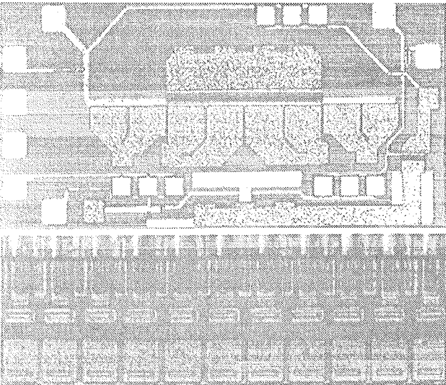
Fig. 14: SiGe-HBT power amplifier and enlarged emitter area
