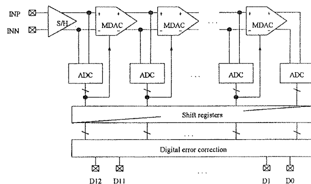
Figure 7. Pipelined ADC for 3rd generation ADSL
