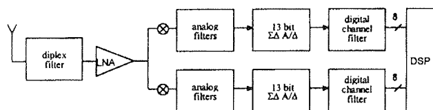
Figure 4. Second generation GSM radio receiver
