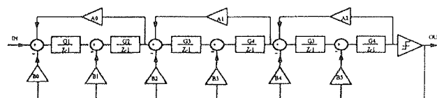
Figure 6. Sixth order SD DAC topology
