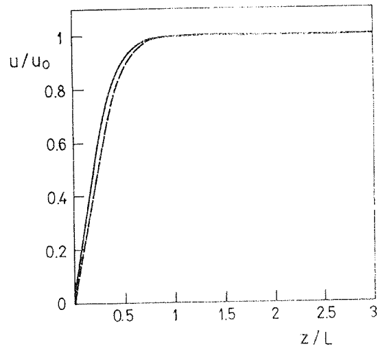
Fig. 8 u(z) = \langle u(x,z) \rangle as a function of z for <<||>> and \gg||<< head on head chevron tip transitions. \theta_t = 0 , q_s/q_0 = 1.01 and the other parameters are the same as in Fig. 6. The \theta(z) = \langle \theta(x,z) \rangle dependence has similar dependence. For the parameters chosen the harmonic approximation [3,4] works well, thus du(x,z)/dx \approx \tan(\theta(x,z)) . u_0 = u(z \gg L) , the domain wall is at z = 0 .
