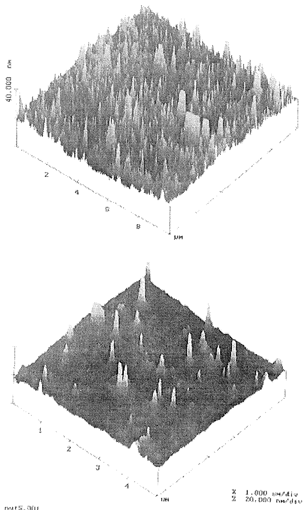
Fig. 2 The AFM images (tapping mode) of a nylon treated surface formed by (a) conventional, (b) "heat quenching" method. In (a) the surface exhibits strong spatial departures from the "ideal planarity" because of the crystalline domains formed within the nylon surface coating. In (b) the crystallisation process is on the average strongly suppressed yielding extremely flat surface.
