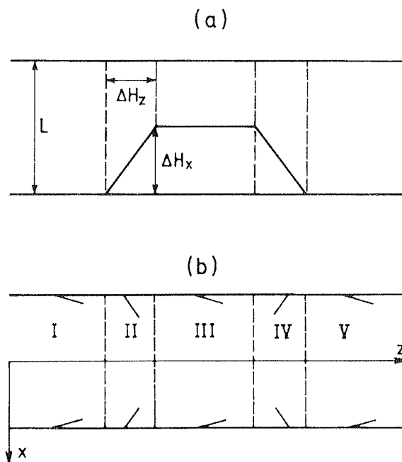
Fig. 4 a) Schematic presentation of the experimental set-up. (b) The spatial variation of the surface slope is within the model imitated by spatially dependent pretilt \theta_t . The sample is divided into regions (i), (ii), (iii), (iv) and (v). The pretilt \theta_t = \theta_p \approx 3^\circ in regions (i), (iii) and (v) is achieved by a nylon surface treatment. The left slope of the region (ii) is simulated by the surface tilt \theta_l = \theta_s + \theta_p \approx 30^\circ and the right one of the region (iv) by \theta_r = -\theta_s + \theta_p \approx -23^\circ .
