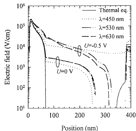
Fig. 2 Calculated electric field profile of the optimized PVI 1 I 2 I 3 N structure for a three-color detector under different monochromatic illuminations and two biases.
