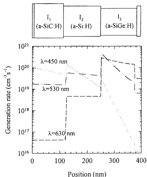
Fig. 1 Generation rate profiles throughout a PI 1 I 2 I 3 N structure for different monochromatic illuminations ( 1 \text{ mW/cm}^2 ).
