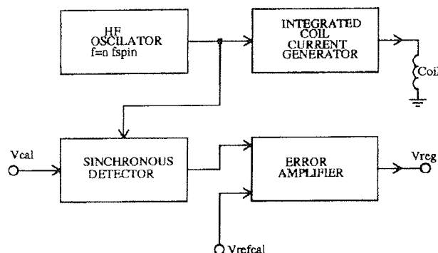
Fig. 3: Block diagram of magnetic sensitivity correction.
