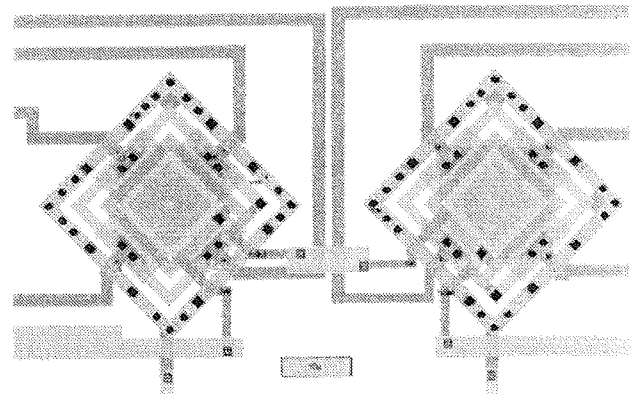
Fig. 2: Hall element pair with integrated coil for reference field generation.
