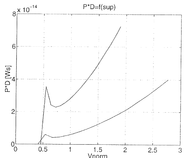
Fig. 2: P \cdot D product as a function of normalized supply voltage
