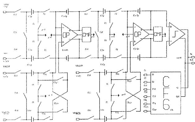
Fig. 3: Simplified circuit diagram of the modulator
