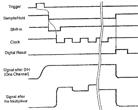
Figure 2: The control signals of the DAQ system and corresponding output from VA1 chip.
