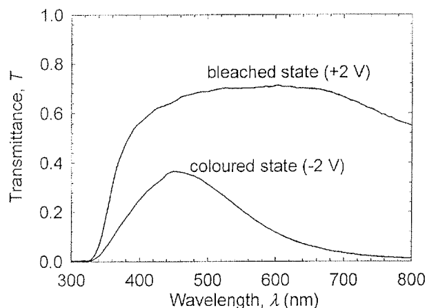
Fig. 2: Transmittances of the EC window in coloured and bleached state
