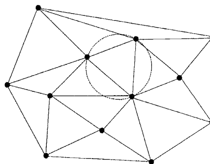
Figure 1 Delaunay triangulation
