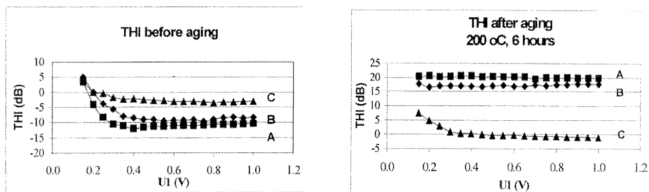
Fig. 5 Third harmonic index (THI in dB) of joints prepared of adhesives Alpha Metals 171 (A), Alpha Metals 181 (B) and ECA 3 (C) on Cu surface before and after aging at 200 ^{\circ}\text{C}
