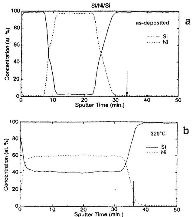
Fig. 8 a, b. AES depth profiles of Si/Ni/Si sandwich layer: (a) as-deposited and (b) after dynamic heating in a DSC instrument at a rate of 40\text{ }^{\circ}\text{C min}^{-1} from room temperature to 320\text{ }^{\circ}\text{C} .
