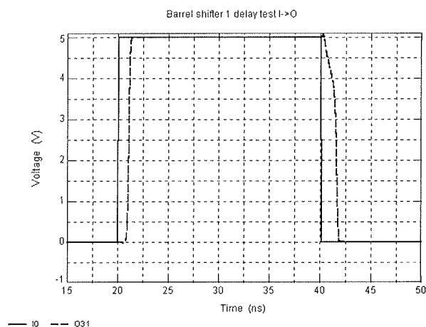
Fig. 16 Signals simulated by SPICE (propagation delay t_{DIO} for barrel shifter with pass transistors).
