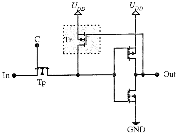
Fig. 6. Output level-restoring buffer with adjacent nMOS pass transistor [4].
