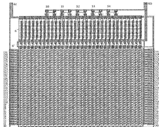
Fig. 12a. Barrel shifters layouts: barrel shifter with pass transistors
