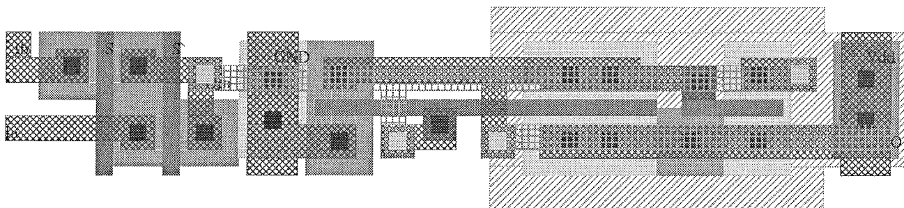
Fig. 13a. Logarithmic shifter basic cells layouts: multiplexer with pass transistors.
