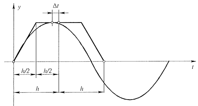
Fig. 5. Frequency warping demonstrated in time domain.
