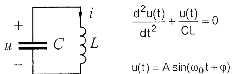
Fig. 4. The circuit in Example 1
