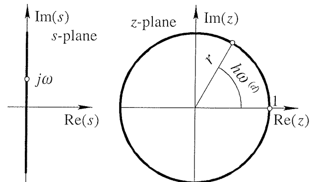
Fig. 2. Map of the ordinate of the s -plane into the z -plane according to the trapezoidal method.
