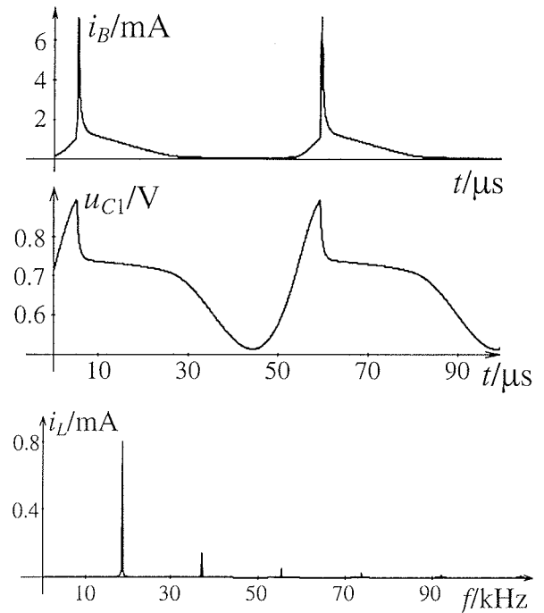
Fig. 8. Base current, base-emitter voltage and the spectrum of the inductor current ( T_{step} = T_{max} = 50 ns)
