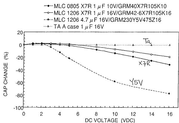
Figure 7: Capacitance versus DC voltage behaviour of different capacitors
