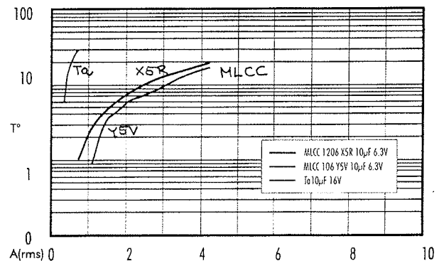
Figure 5: Temperature rise of different capacitors working at 100 kHz
