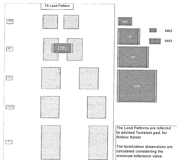
Figure 12 . MLCC to Ta matching sizes
