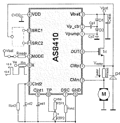
Fig. 3 Application circuits of the DC Motor regulator in operating mode 1 (left) and operating mode 2 (right)
