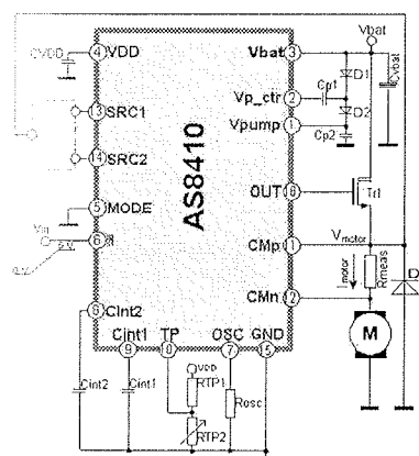
Fig. 3 Application circuits of the DC Motor regulator in operating mode 1 (left) and operating mode 2 (right)
