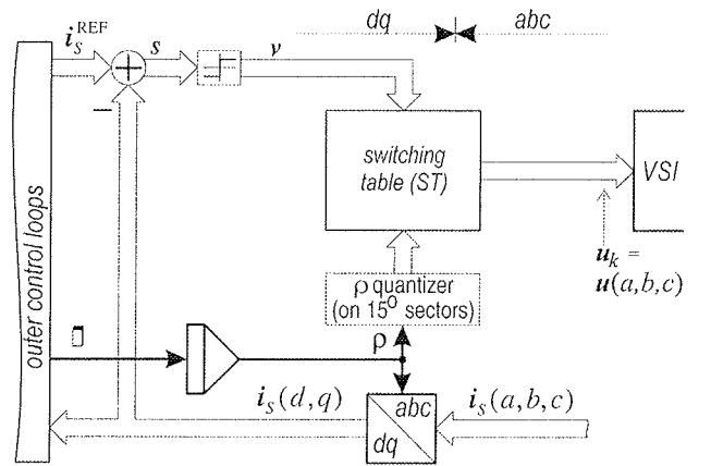
Fig. 3: Realization of decoupled SCC.
