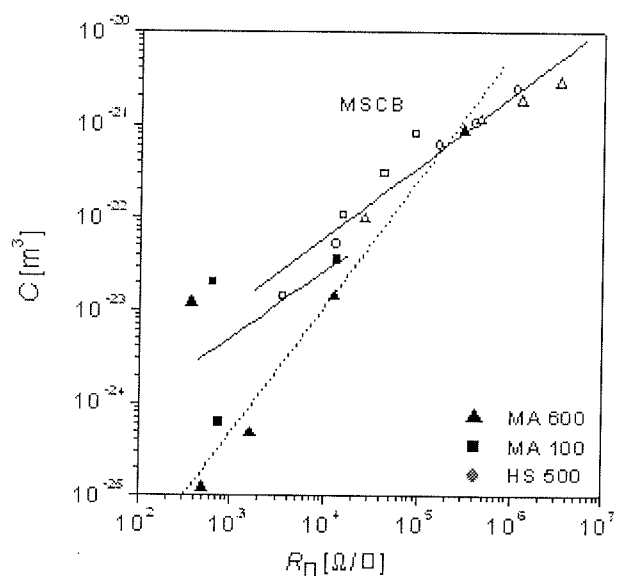
Fig. 3. Noise intensity C versus sheet resistance R_{\square} for carbon black/polyesterimide (open symbols) and carbon black/polyimide (full symbols – these data refer to results of Fu et al /28/) resistors
