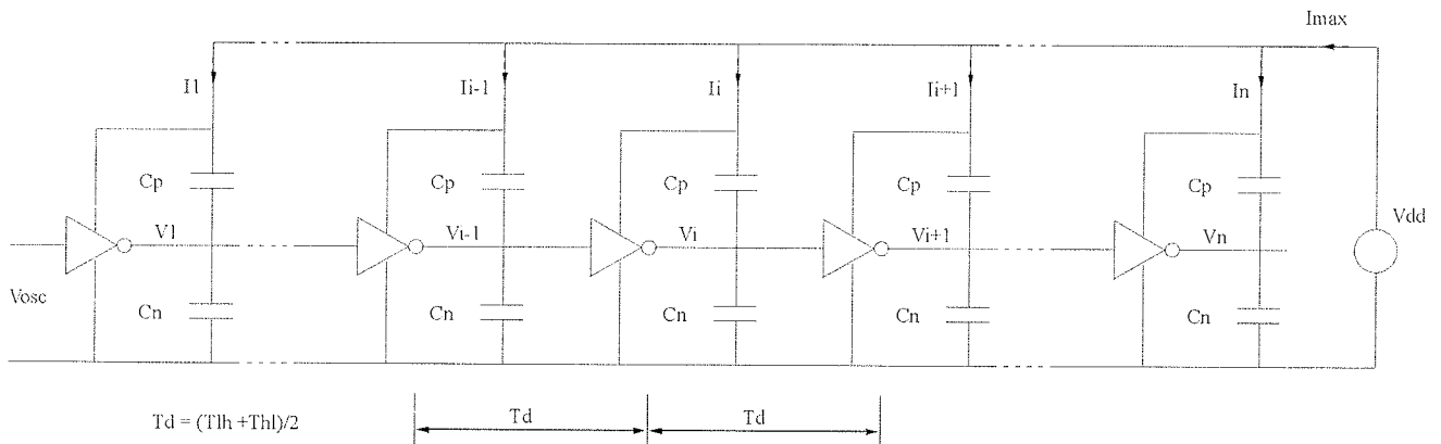
Figure 2: The distributed clock driver as the chain of inverting buffers
