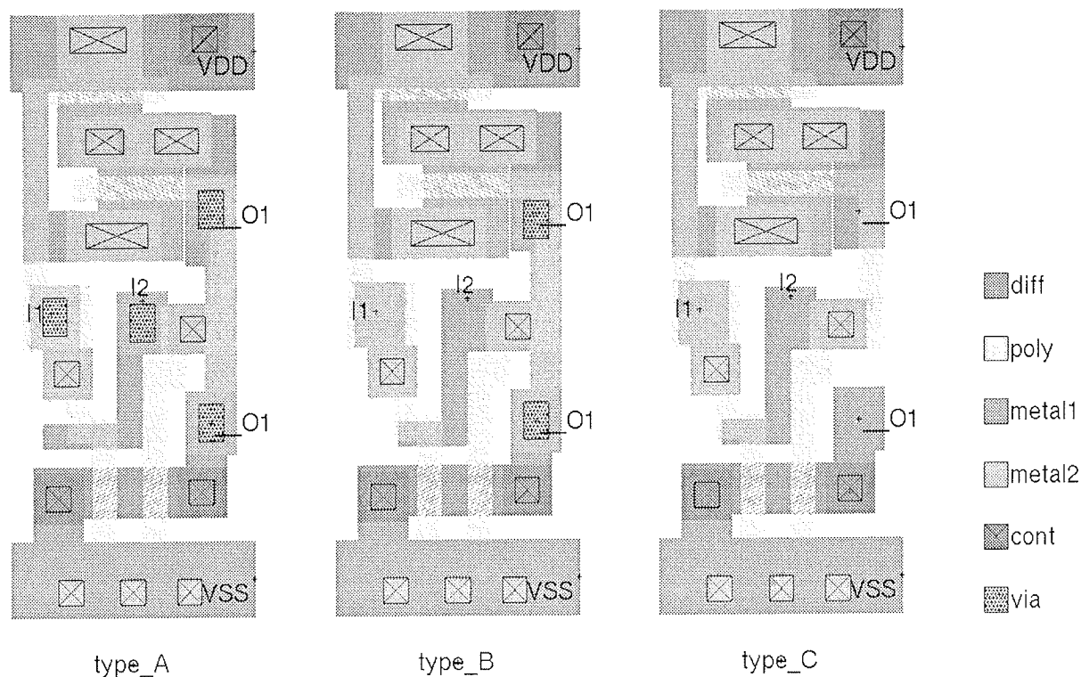
Figure 1: Three versions of NAND2: (A) every pin is accessible from channel, (B) only output is accessible from channel, (C) all connections must be made in metal1. Well is omitted to improve readability.
