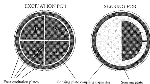
Fig. 1a: PCB layout for absolute 360 degree angle measurement system
