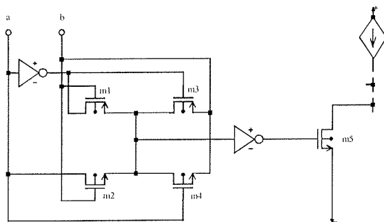
Figure 5: EXnOR logic
