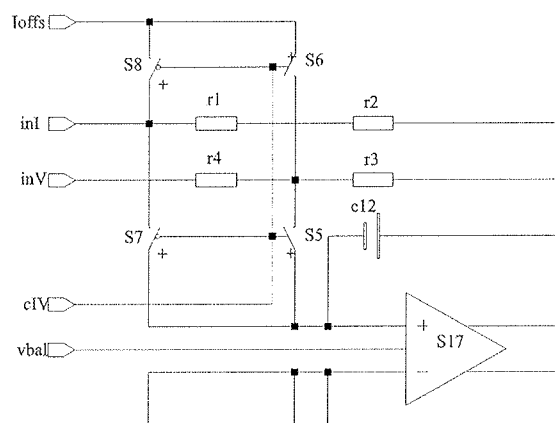
Figure 2: The AFE signal-channel half of the symmetrically-balanced stage. The current input \text{inI} or the voltage input \text{inV} is selected by the \text{cIV} signal. The \text{Ioffs} input current is selected for the offset correction of the AFE. Integrated diodes are connected from \text{inI} inputs to the substrate (VDD) in reverse polarity. Each channel has two photodiodes.
