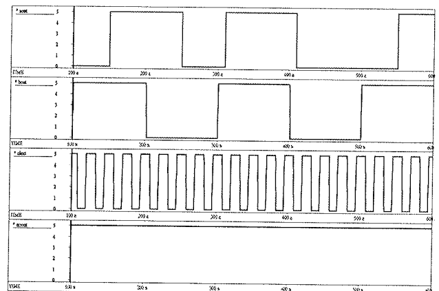
Figure 4a: Error function: principle of operation. External clock frequency is f_{ext} > 4FD.f_{sin} . Error is not detected if there is clock edge between track A and track B.
