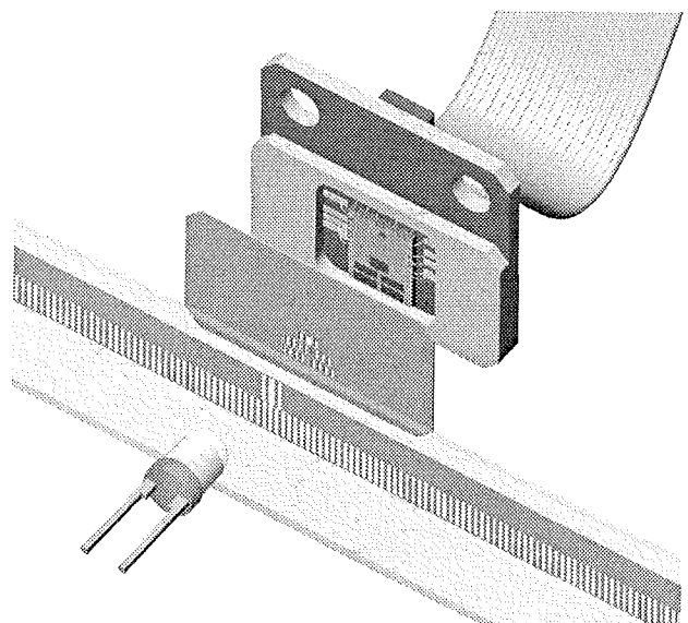
Figure 9: Opto-ASIC in linear-incremental-position application
