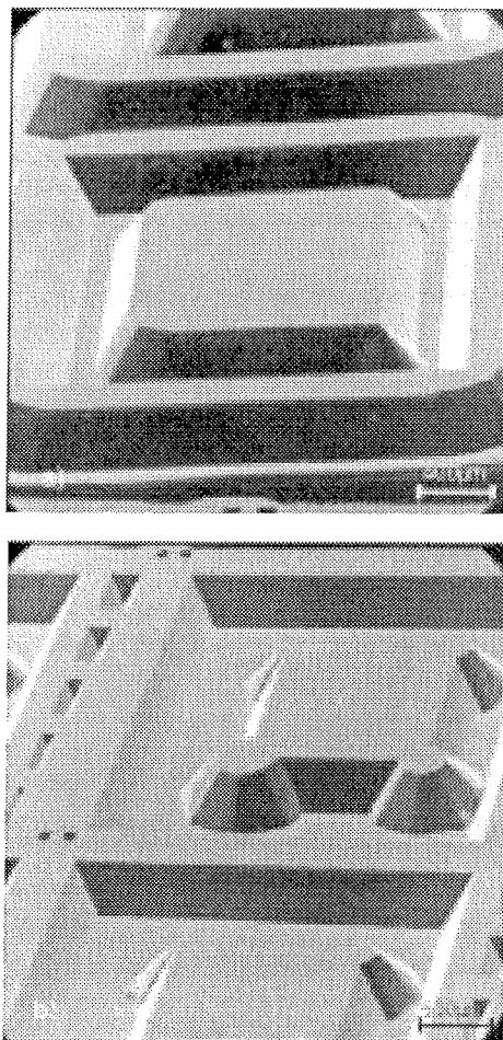
Figure 15: Compensation of convex corners in realization of bossed diaphragms.
