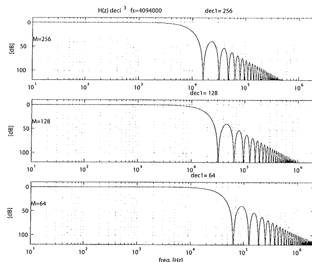
Figure 7: Programmable decimator frequency characteristics
