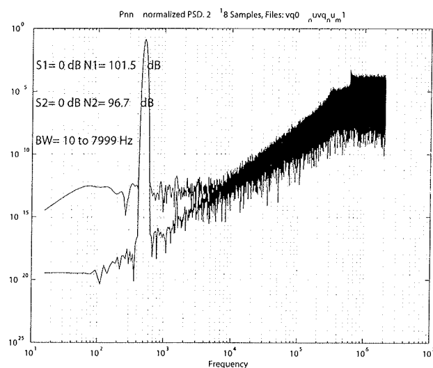
Figure 6: PSD of a bit stream
