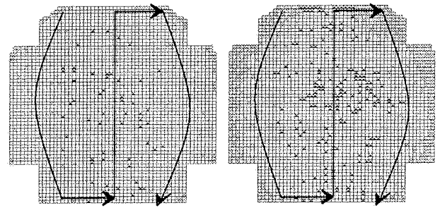
Figure 5: Best and worst-case inking wafer map for three passes inking algorithm.
