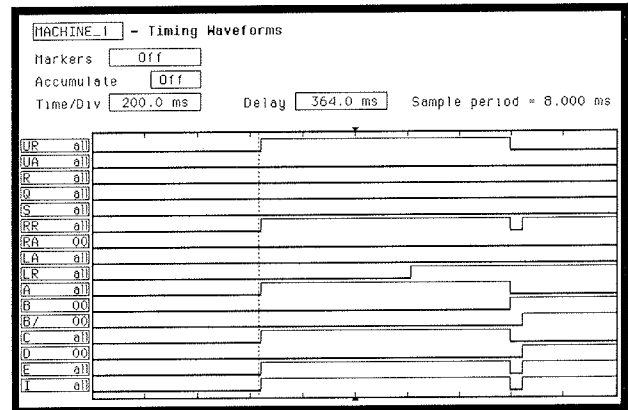
Figure 12: Hazard on signal RR in McMillan's DME cell
