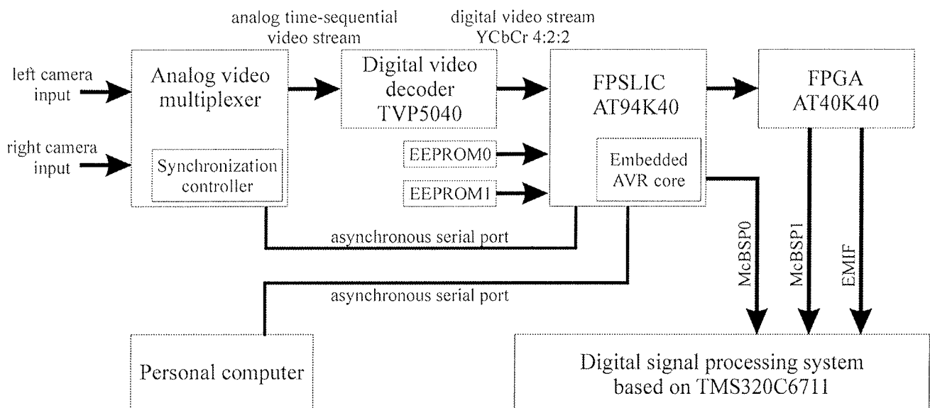
Figure 7: Block scheme of the capture unit.
