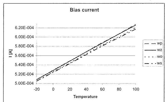
Fig. 13: Bias current
