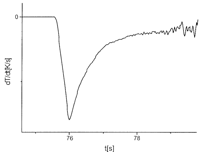
Figure 3: Time derivate of the temperature of the probe, the cooling part of the slope.
