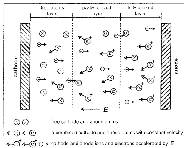
Fig. 3: The arc layers.
