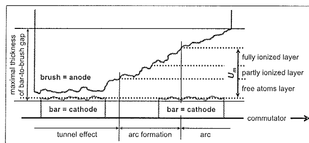
Fig. 2: The formation of the electric drawn arc during the commutation.
