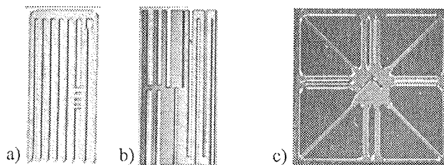
Fig.5. Three different designed and fabricated monolithic silicon optical benches with fibre grooves and reflecting mirrors (a,b-size 5 \times 10 \text{ mm}^2 , c-size 10 \times 10 \text{ mm}^2 ).
