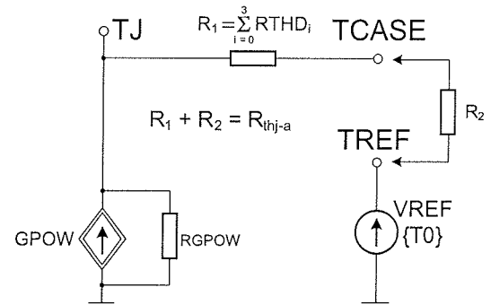
Fig. 4. The thermal model of the SiC Schottky diode for d.c. analysis
