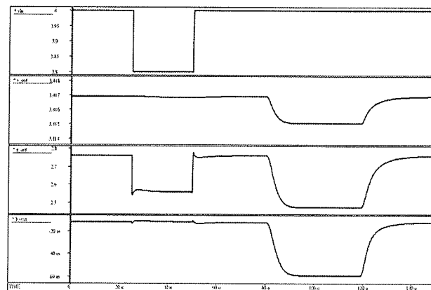
Fig. 5. Simulated response of regulator in the case of 100 \mu F blocking capacitor
