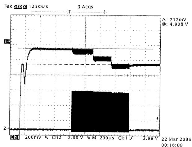
Fig. 6. System response data in the neighbourhood of the ideal conditions
