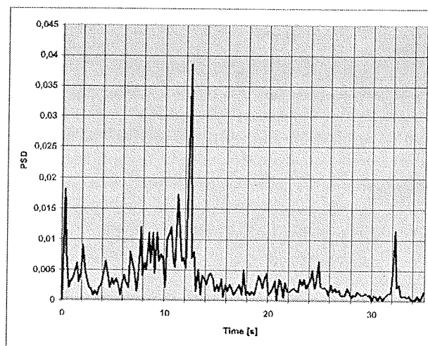
Fig. 8: Power spectral density of the Bora in the Gulf of Trieste.
