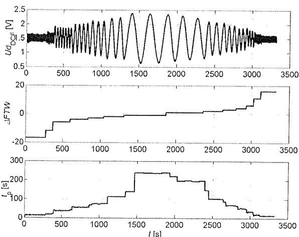
Fig. 5: Demodulated signal from the DCF77 transmitter U_{d\_DCF} and the time of one period at different settings of the DDS FTW of the DCF77 receiver \Delta FTW , \Delta FTW = FTW - 16643112 .
