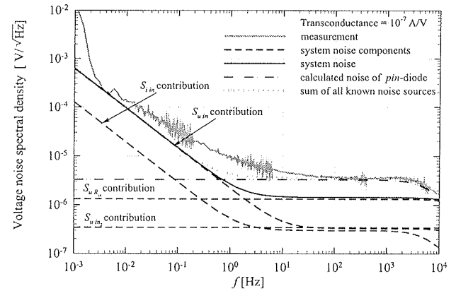
Fig. 12: Noise voltage density spectrum, measured at the SR570 output, of the a-Si:H pin diode at forward current bias of 420 nA. The contribution of individual noise sources of the measurement system and the known noise components of the pin diode are added for comparison. The observed excess noise is 1/f noise component of the pin diode.
