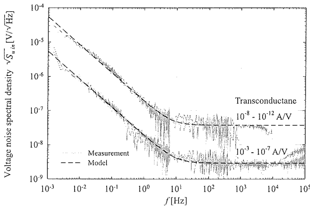
Fig. 8: Noise power density spectra of the equivalent input noise voltage source of SR570 at different sensitivities, extracted at 50 \Omega input termination.
