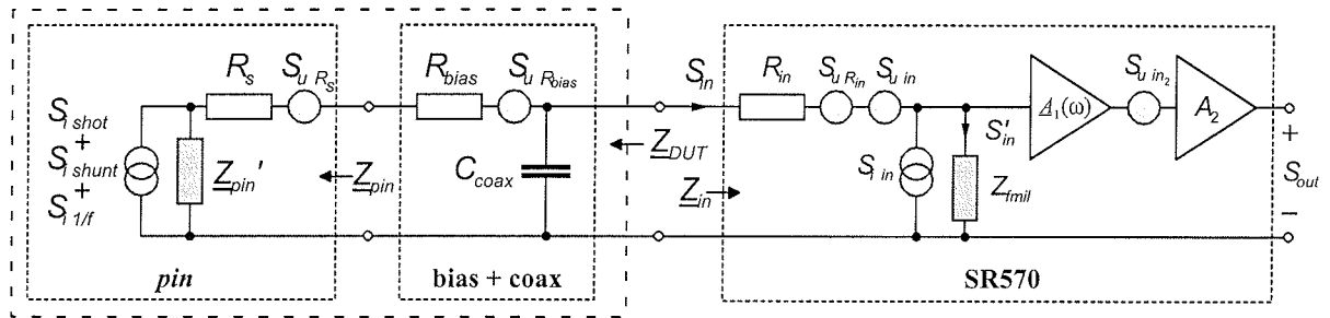
Fig. 11: Noise model of measurement system including a-Si:H pin diode, bias circuit, coaxial cable connection and SR570 transconductance amplifier.
