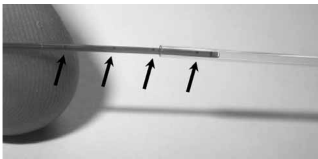
Fig. 11: Example of an 840 \mu\text{m} OD instrumented catheter designed by FISO Technologies for multiple point temperature sensing compatible with RF/MW hyperthermia therapy or thermal ablation. Arrows show the positions of four GaAs sensors.
