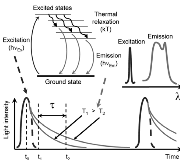
Fig. 1: Schematic description of the fluorescence decay technology. Electronic transitions (top left), typical excitation and emission spectra (top right), reflected light intensity with time (bottom).
